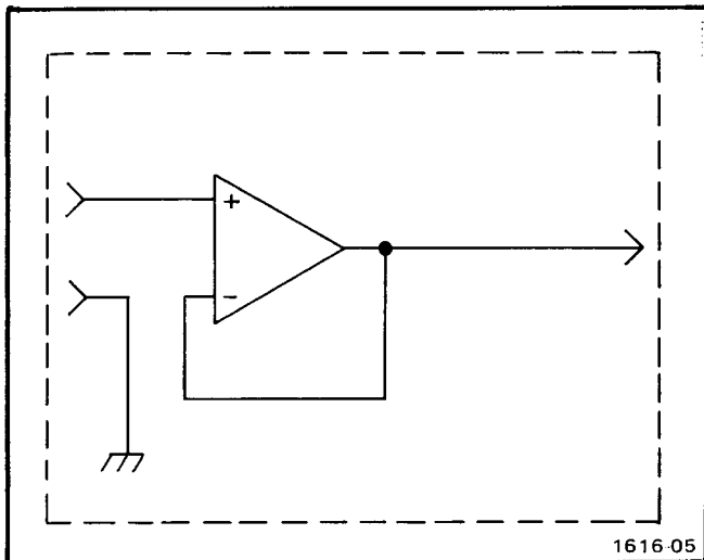
Fig. 1-5. X1 Non-inverting amplifier (follower).
